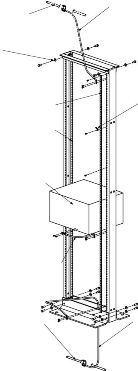
Figure 1 - Properly Grounded/Earthed Rack (Back of Rack Shown)
