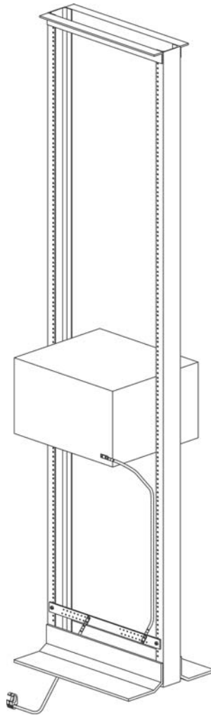
Figure 2 - Retrofit Rack Grounding/Earthing
